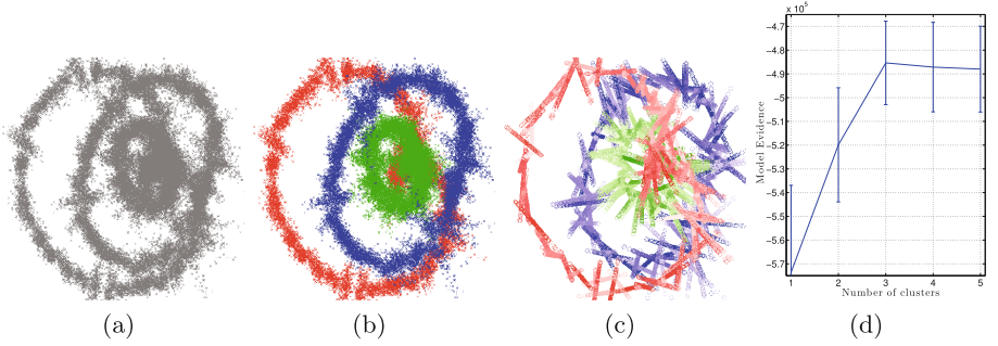
Fig. 2. Clustering and mode estimation of synthetic point sets. (a) overlay of 750 point sets, (b) corresponding color separated ground true clusters, (c) estimated labels (colors), GMM centroids showing local modes of variations, (d) lower bound \mathcal{L} on the model evidence versus number of clusters, indicating J = 3 as the optimal number (Color figure online).
