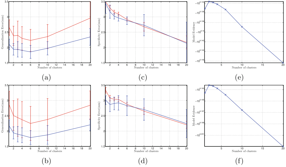
Fig. 4. Quantitative results for models trained by clustering normal-HCM (top row) and normals-PH (bottom row) cases versus number of clusters, (a-b) Generalization errors as distances between the model projected and original test sets (red), and vice versa (blue), (c-d) Specificity errors as distances between model generated and training point sets (red), and vice versa (blue). (e-f) show the model evidence (Color figure online).
