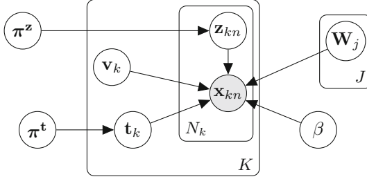
Fig. 1. The graphical representation of the proposed model; shaded and hollow circles represent observed and latent variables, respectively, arrows imply the dependencies and plates embrace numbered incidences of events.
