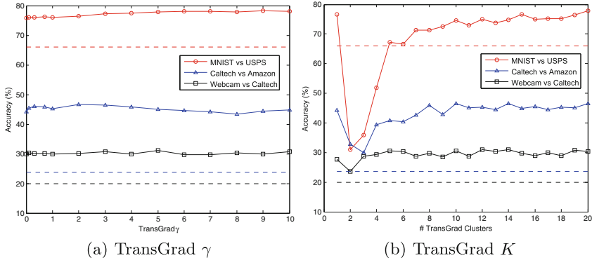
Fig. 3. Effect of different \gamma values and number of GMM clusters in the TransGrad step of our framework on the final performance of the pipeline for three cross-domain experiments. The dashed line shows the baseline accuracy for each experiment.
