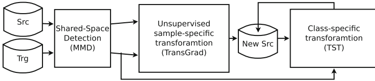
Fig. 2. The Transductive Transfer Machine (TTM).
