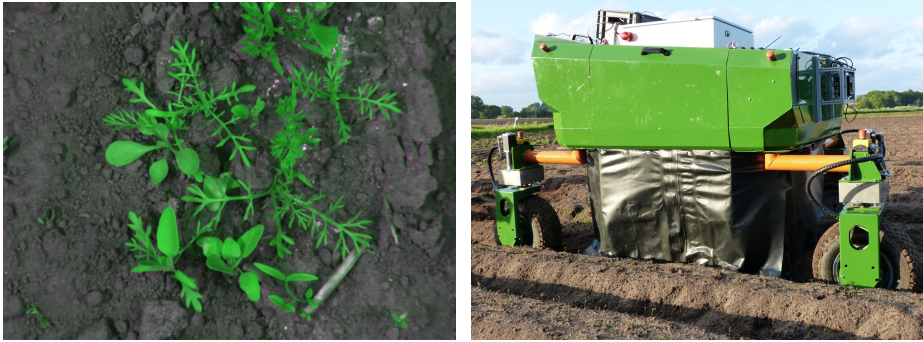
(a) Sample image from dataset. (b) Field robot used for dataset acquisition.
