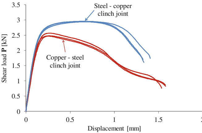
Fig. 11 Shear characteristics of steel and copper clinch joint
