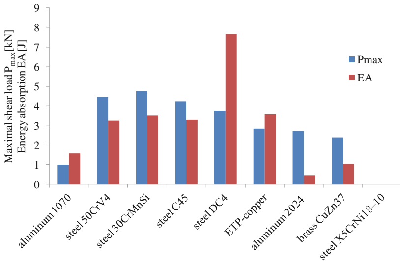
Fig. 18 Strength properties of clinched joints for different kind of joined materials
