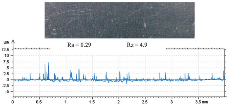
Fig. 35 Picture of surface and profile roughness parameters for 50CrV4 steel sheet ( R_a and R_z in \mu\text{m} )
