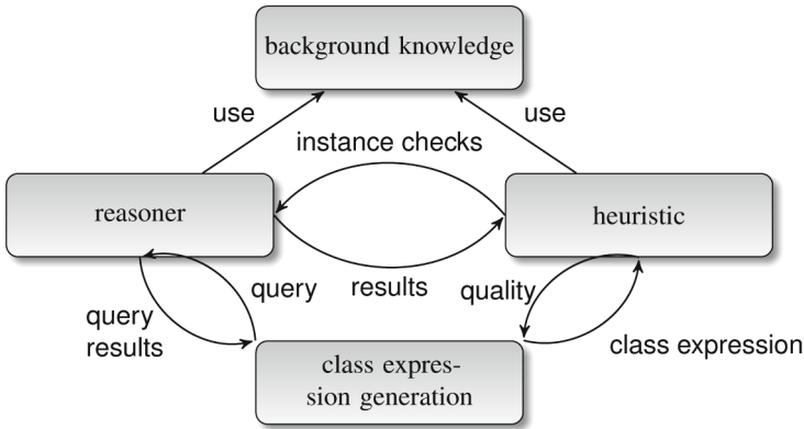
Fig. 1. Outline of the general learning approach in ETL: Class expressions taking the available background knowledge into account are generated and evaluated in a heuristic with respect to the target learning problem. Figure adapted from [14].
