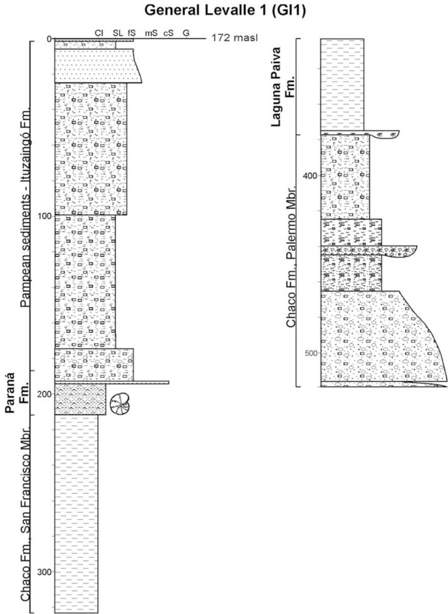
Fig. A.5 Log of General Levelle 1 borehole
