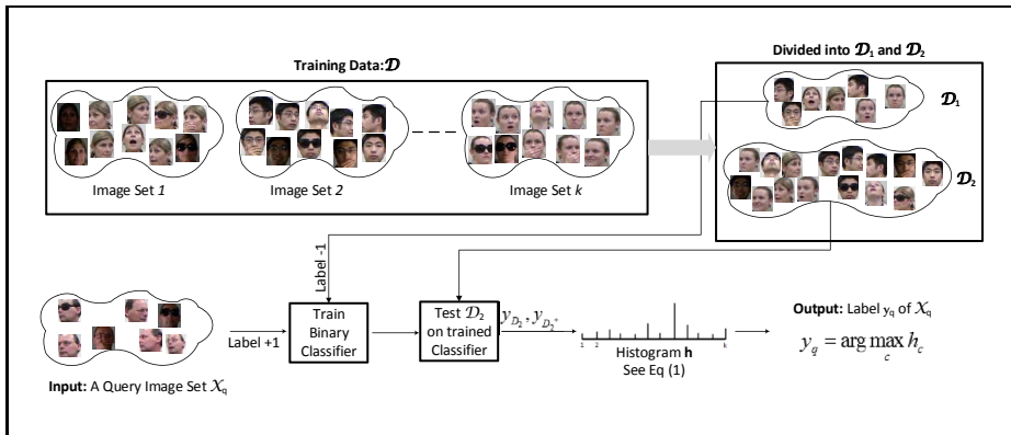
Fig. 1. Block diagram of the proposed method. Training data is divided into two sets \mathcal{D}_1 and \mathcal{D}_2 . \mathcal{D}_1 contains uniformly randomly sampled images from all classes such that the size of \mathcal{D}_1 is the same as the size of the query image set \mathcal{X}_q . A binary classifier is trained, with images of \mathcal{X}_q (labeled +1) and \mathcal{D}_1 (labeled -1). The classifier is then tested on the images of \mathcal{D}_2 . Knowing the class labels of images of \mathcal{D}_2 which are classified +1, we formulate a histogram (see Eq. 1), which is then used to decide about the class of \mathcal{X}_q . See a toy example in Fig 2 for illustration.
