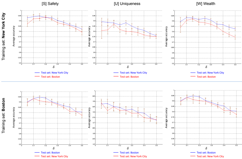
Fig. 4. Each figure shows the mean accuracy of the classification for different values of the \delta parameter. The blue line represents performance reported on images from the same city as the training data. The red line represents the performance reported on images from a different city than those used for training.
