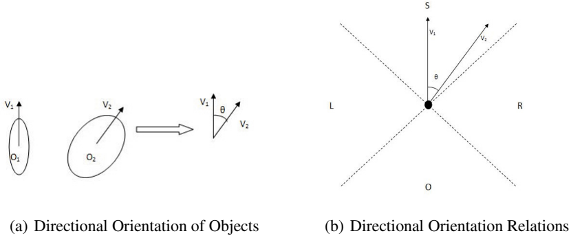
Fig. 1. (a) Egocentric Directional Orientation of Objects (b) Egocentric Directional Orientation Relations
