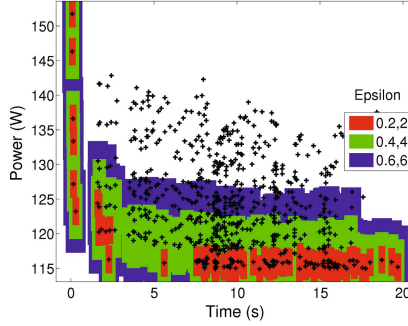
Fig. 2. Illustration of the points comprising a relaxed Pareto front for different values of \epsilon (SPAPT adi problem, Intel Xeon Phi; see Section 6.1). The points within each shaded region belong to the relaxed Pareto front obtained from (4).
