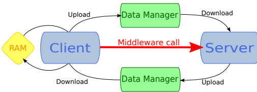
Fig. 2. Automatic transfers during a GridRPC call
