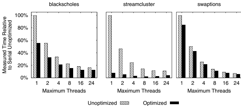
Fig. 7. ParaShares pinpoint inefficiencies that lead to significant opportunities for optimization. With the extremely targeted profiling provided by ParaShares, we were able to improve benchmark performance by up to 92% through source code changes less than 10 lines long.
