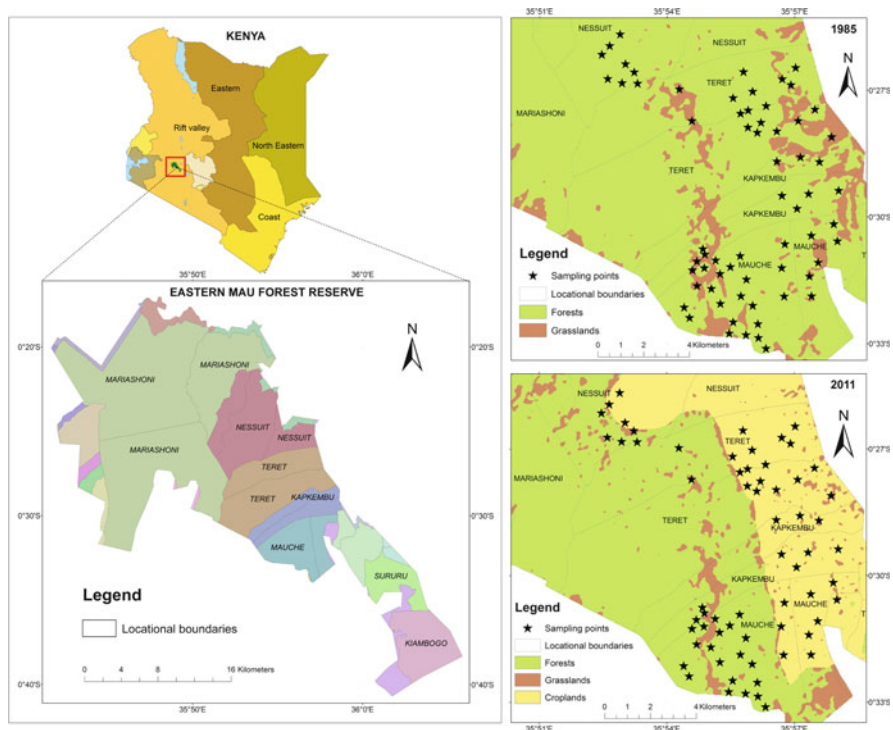
Fig. 6.2 Geographical location of the study area and sampling points. The sampling points are superimposed on the land cover maps of 1985 and 2011 (on the right ) that were derived from digital classification of Landsat TM imagery
