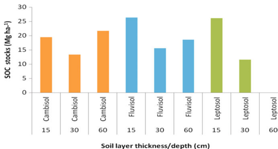
Fig. 17.4 The mean SOC stocks of the major soil types to the soil depth of 60 cm
