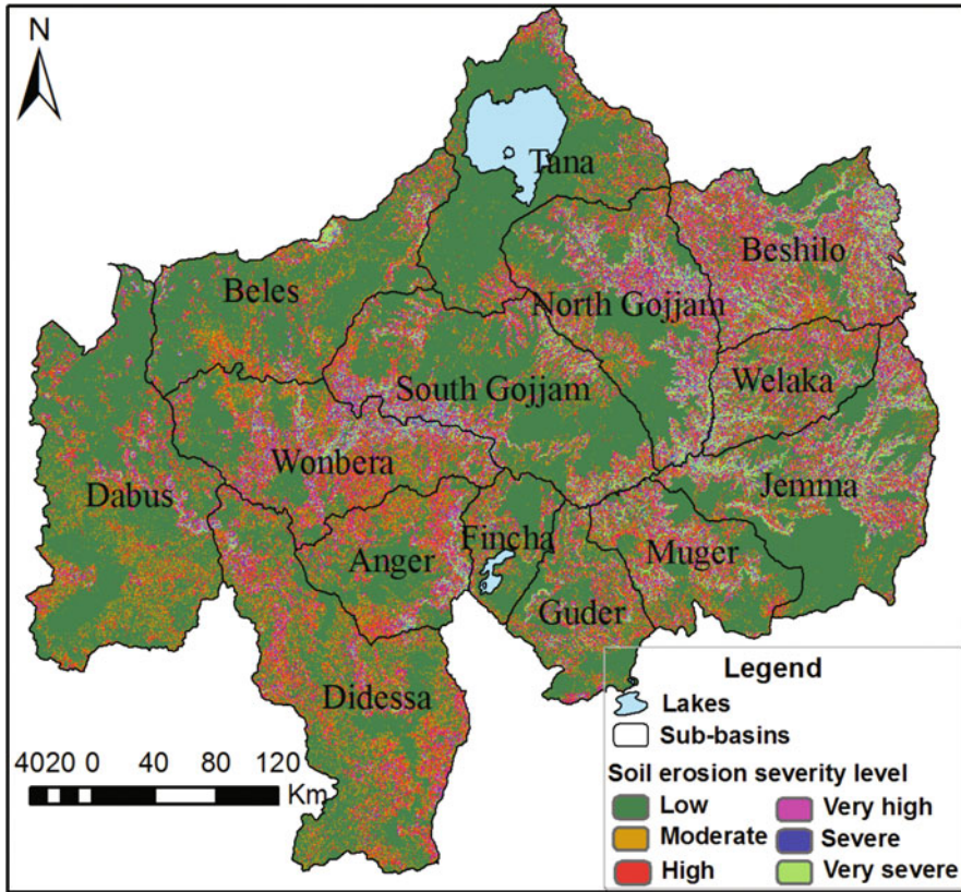
Fig. 7.7 Potential soil erosion hazard for 50 % SOM reduction in the Upper Blue Nile River Basin
