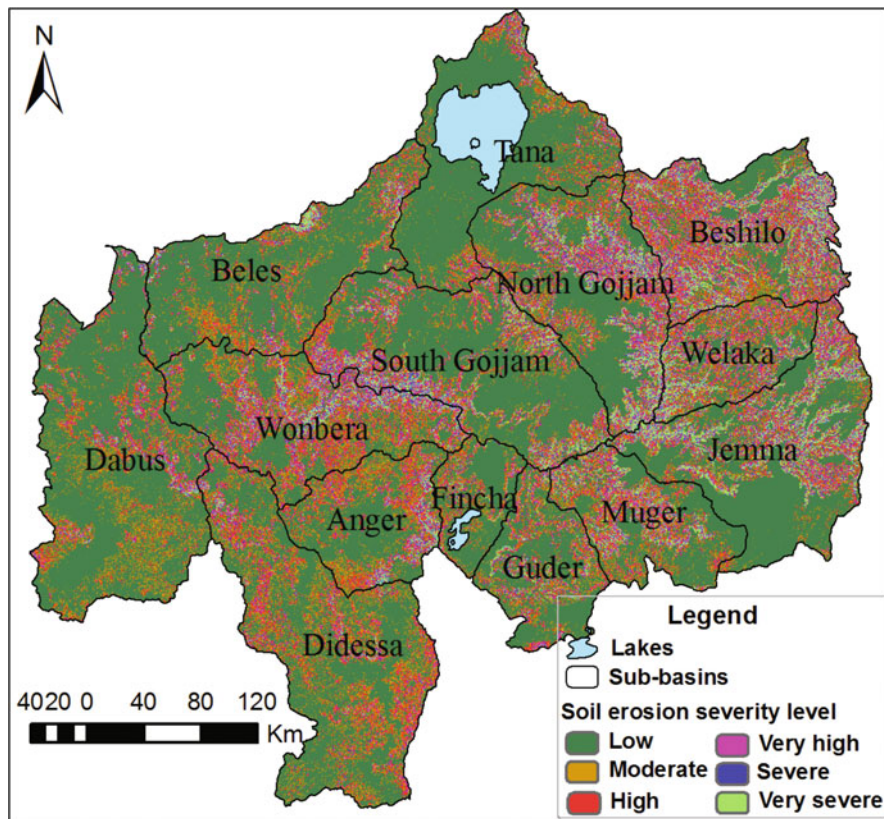
Fig. 7.6 Potential soil erosion hazard for 20 % SOM reduction in the Upper Blue Nile River Basin
