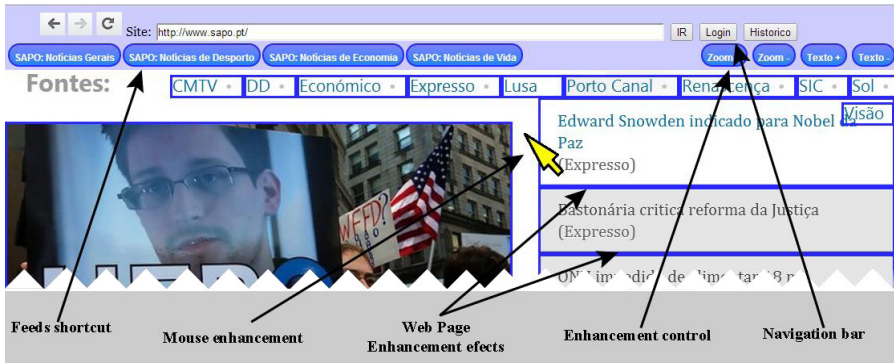
Fig. 2. AdaptNow interface visualization of an enhanced webpage
