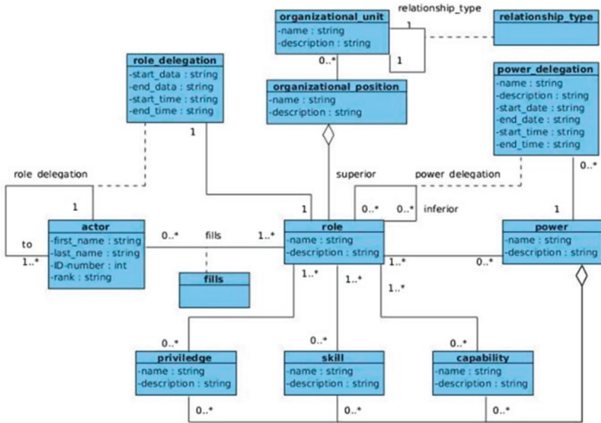
Fig. 3 Role model
