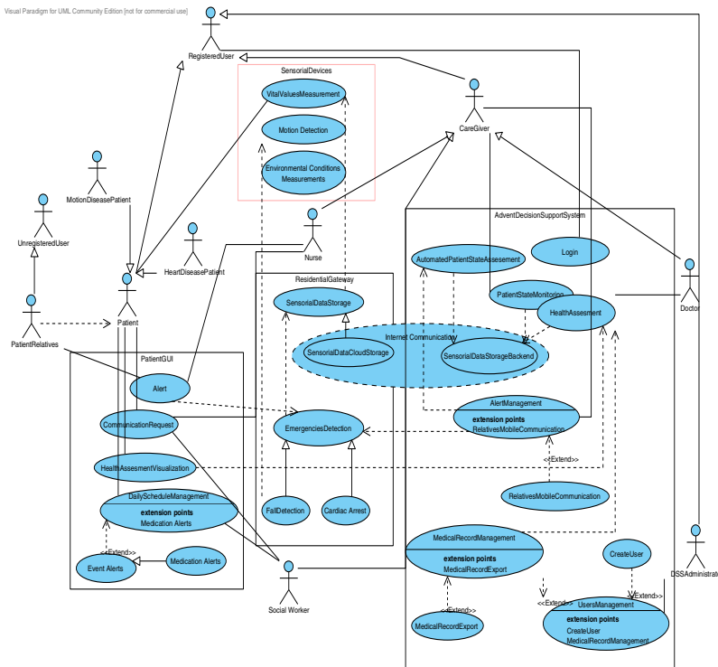
Fig. 1. ADVENT Requirements Use Case Diagram
