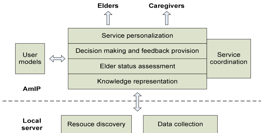
Fig. 5. ADVENT middleware high-level architecture
