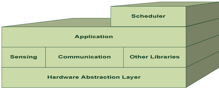
Fig. 4. A high level TinyOS based Software Stack Architecture
