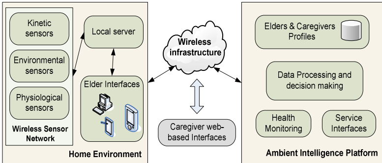
Fig. 2. ADVENT system architecture block diagram
