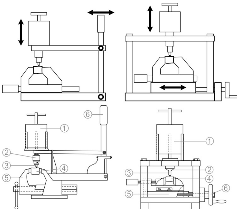
Fig. 1 Basic mechanisms as well as exemplary sketches of the two main forms of test apparatus in use. Left Type 1, original design CERCHAR-type testing apparatus. Right Type 2, the modified CERCHAR apparatus as reported by West (1989). 1 mass, 2 pin chuck/guide, 3 stylus, 4 specimen, 5 vice, 6 lever/hand crank
