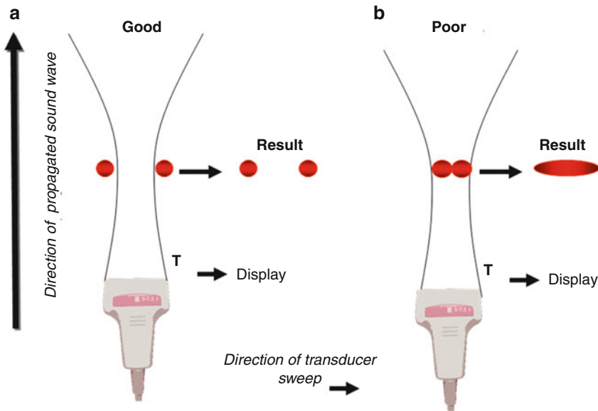
Fig.2.13 Lateral resolution is optimized when beam width is narrow enough to fit between two objects equidistant from the transducer. In (a) the objects would be correctly displayed as separate objects. In (b) the beam width is too thick to fit between the objects and they would be displayed as a single “blurred” focus
