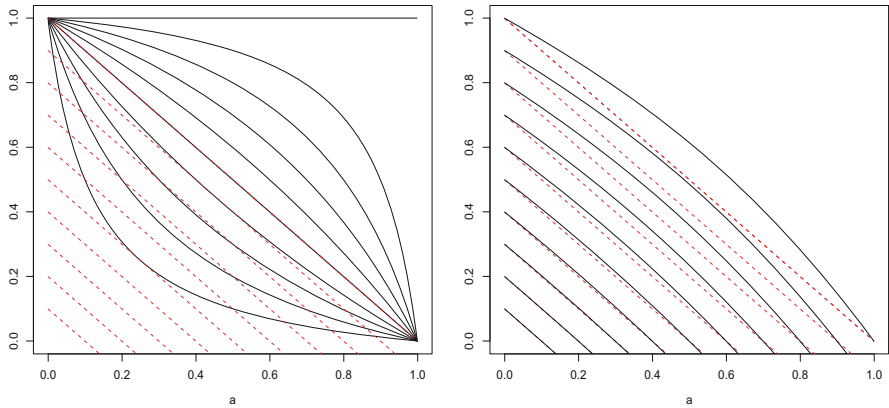
Fig. 2 Level curves L_c for the logistic ( left panel ) and hyperbolic sine ( right panel ) transformations. The red (dotted) lines are level curves for a + b , while the black (solid) lines are level curves for a \oplus b , where c = 0.1, 0.2, 0.3, 0.4, 0.5, 0.6, 0.7, 0.8, 0.9, 1.0
