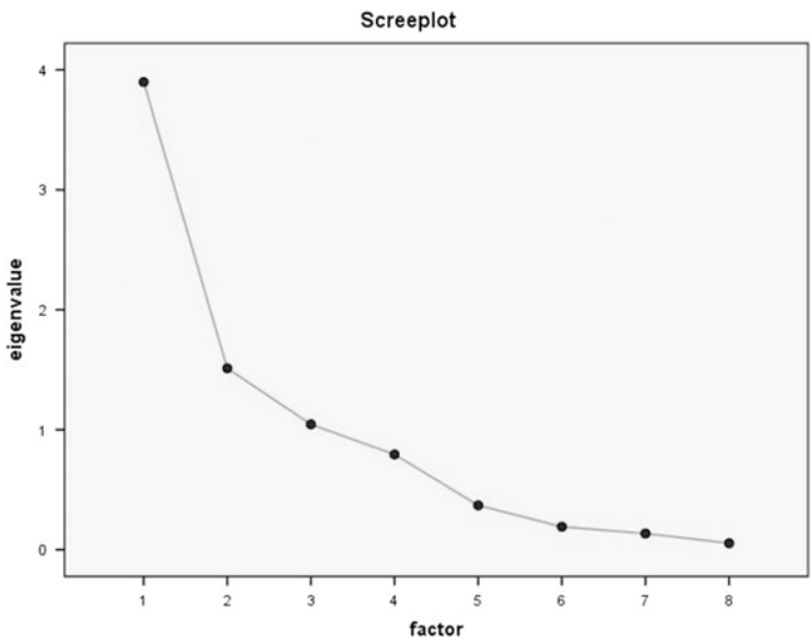
Fig. 4 Screplot (model 2)
