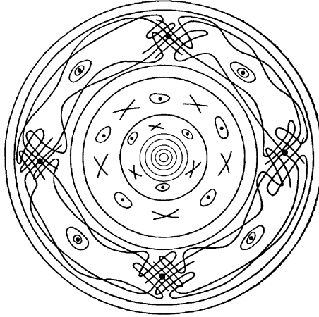
Fig. 3. More fixed points... after [1]
