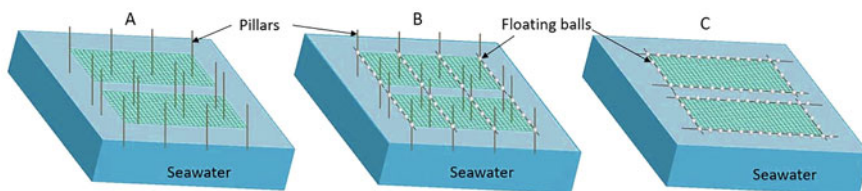
Fig. 2 Three offshore farming techniques of seaweeds, namely pillar type (a), semi-floating raft (b), and full floating raft composed of long rope and floating balls (c). Source: Modified from Zhang et al. (2022), Open access article
