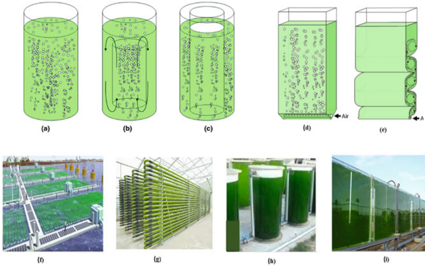
Fig. 6 Illustration showing different microalgae closed cultivation systems. (a) Normal column reactor, (b) Column reactor with concentric airlift (c) Annular reactor, (d) Flat plate aeration tube (e) FPA photobioreactor (f) Offshore cultivation (g) Tubular reactor (h) stirred tank (i) Flat reactor. Source: Modified from Pal and Satpati (2018) and Yusoff et al. (2019)
