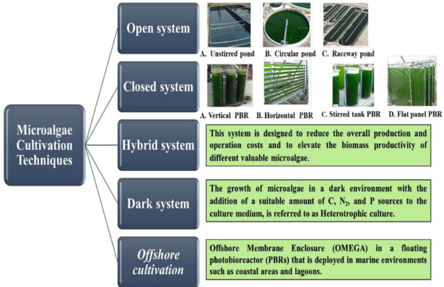
Fig. 4 Different microalgae cultivation systems including open ponds (A. unstirred pond; B. circular pond; C. raceway pond), closed photobioreactors (A. vertical PBR; B. horizontal PBR; C. stirred tank PBR; D. flat panel PBR), and hybrid systems, in addition to dark and offshore systems
