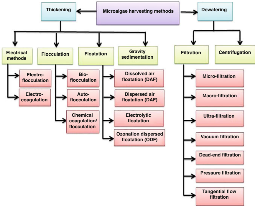
Fig. 1 Schematic diagram showing the various methods used for harvesting microalgae
