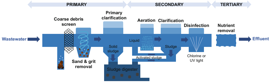
Fig 1 Schematic diagram of three main stages of the conventional wastewater treatment process
