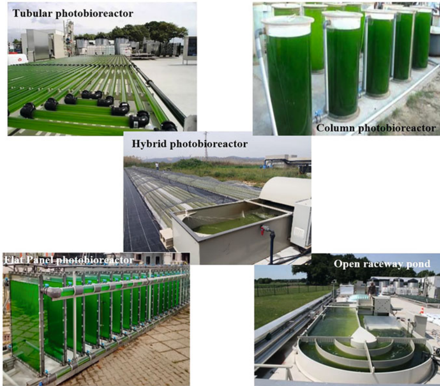
Fig. 2 Commonly used photobioreactor systems for the growth of microalgae. Sources: the open access references (Ahmad et al. 2021; De Vree et al. 2015); Lindblad et al. (2019) with License Number 5570200199862; and Belohlav et al. (2021) with License Number 5570190519426
