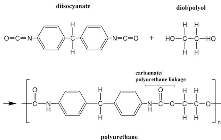
Fig. 3 Schematic reaction mechanism for the synthesis of polyurethane. A polyol, an alcohol with at least two reactive hydroxyl groups, and a diisocyanate or polymeric isocyanate react to produce polyurethane under the presence of suitable catalysts. Additives, e.g., short polyols as chain extenders or blowing agents, e.g., water to obtain foams, could be added to manipulate the properties of the end-products
