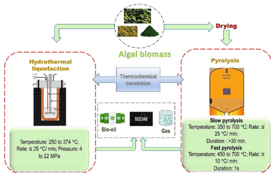
Fig. 1 Hydrothermal liquefaction and pyrolysis as common routes of thermochemical conversion of algal biomass. Data in the figure are extracted from Aliyu et al. (2021)
