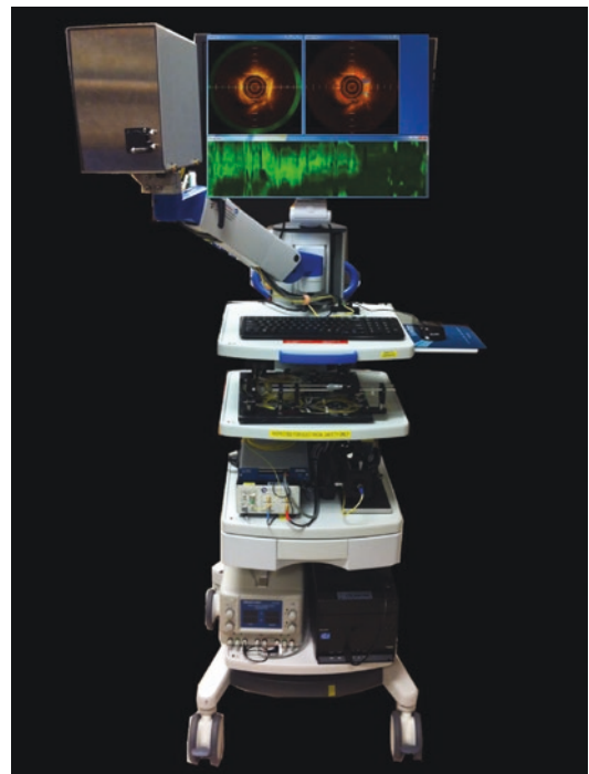
Fig. 22.1 AF-OCT prototype
