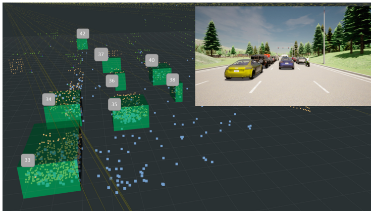
Fig. 1. Performance of the DAMOT method in a traffic jam use case in AD PerDevKit dataset. Tracked objects are shown as green Bounding Boxes.
