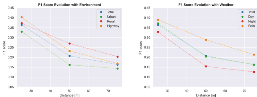
Fig. 4. Evolution of F1 score with respect to the distance evaluated over the different environments (left) and climate (right) scenarios offered by AD PerDevKit.
