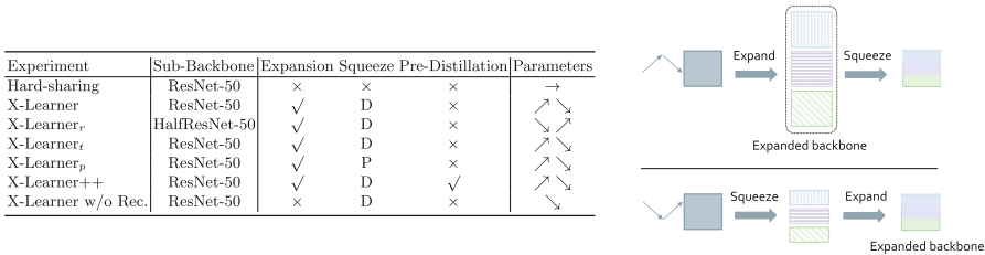
Fig. 4. Differences among X-learner variants. We conduct different ablation study of X-Learner. Pre-distillation refers to applying extra supervisions from single-task single-source pre-trained models as is introduced in X-Learner++. In the Squeeze column, we denote distillation by D and pruning by P if there is a squeeze stage present in the pipeline. The change of the parameter can refer to the figure on the right.
