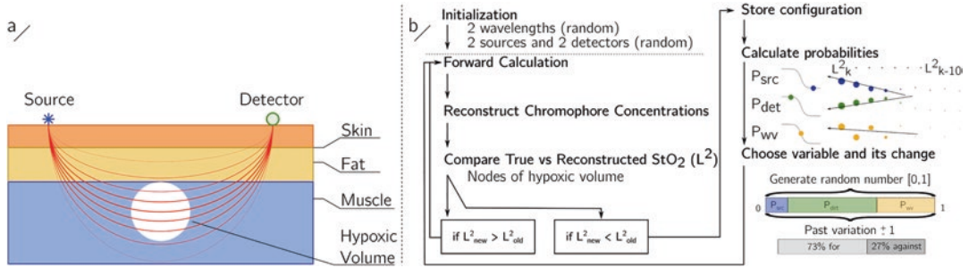
Fig. 1 (a) Representative geometry of the finite element tissue mesh and hypoxia placement. (b) Outline of the SGDm algorithm
