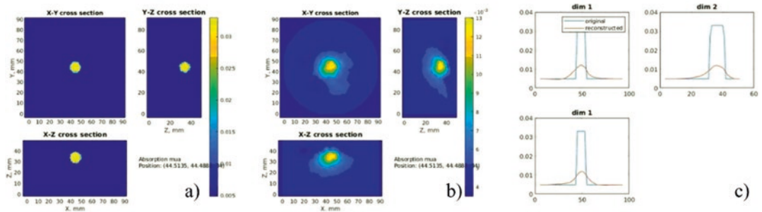
Fig. 5 NIROT imaging of a single inclusion inside the liquid phantom. Expected location of the inclusion (a) shown as distribution of absorption coefficient, and the
