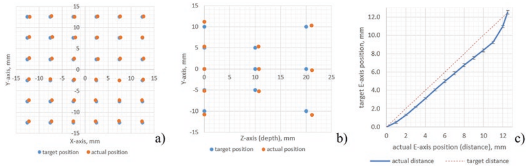
Fig. 4 Comparison of target and actual position of inclusion in cross (a) and longitudinal section (b). Average distance between two inclusions (c)
