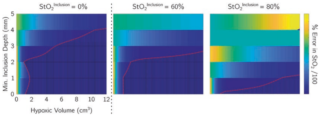
Fig. 2 Percent error in reconstructed StO_2 for different minimum inclusion depths (top of hypoxic sphere) and hypoxic volumes, for three different inclusion StO_2 . The
