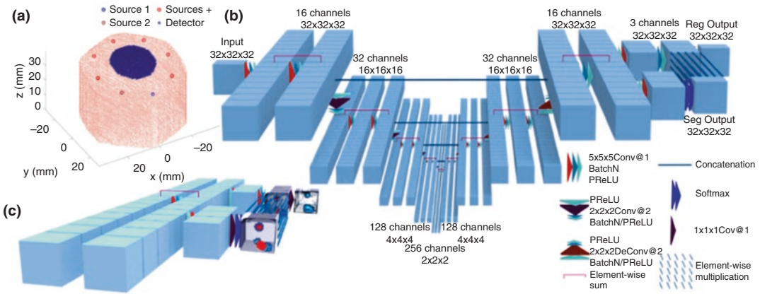
Fig. 1 (a) Mesh of modelled preterm infant head surface illustrating the source-detector placement. (b) Schematic illustration of the hCNN (c) Magnification of the last hCNN layers
