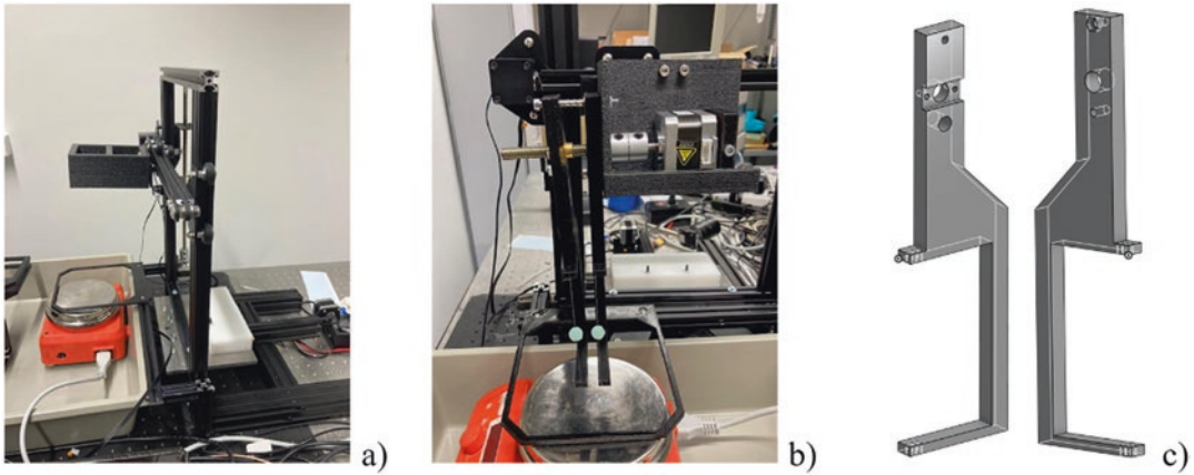
Fig. 3 Moving stage without inclusion holder seen from the side (a), the same stage with the holder and 2 inclusions, front view (b), and the CAD of the left and right holders (c)
