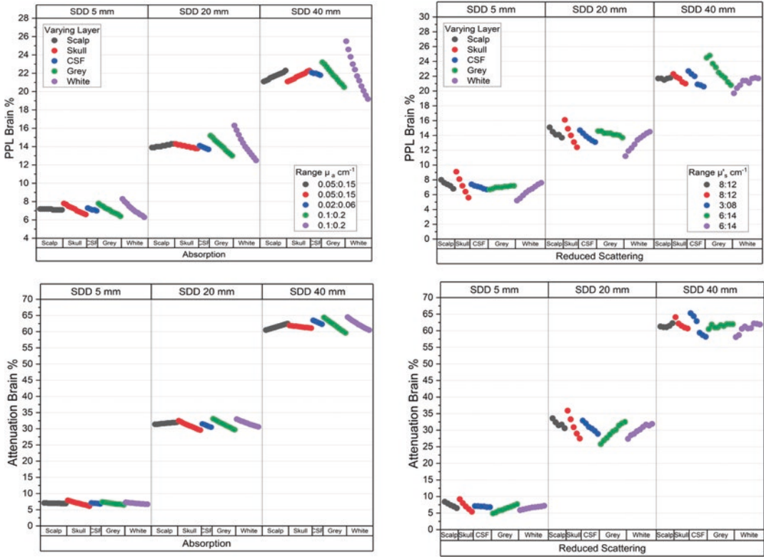
Fig. 2 Scatter plots of the PPL (top) and Attenuation (bottom) relative to the brain photons by varying the scattering (right) and the absorption (left) of a specific layer. From left to right, in every sub-groups of coloured dots,
