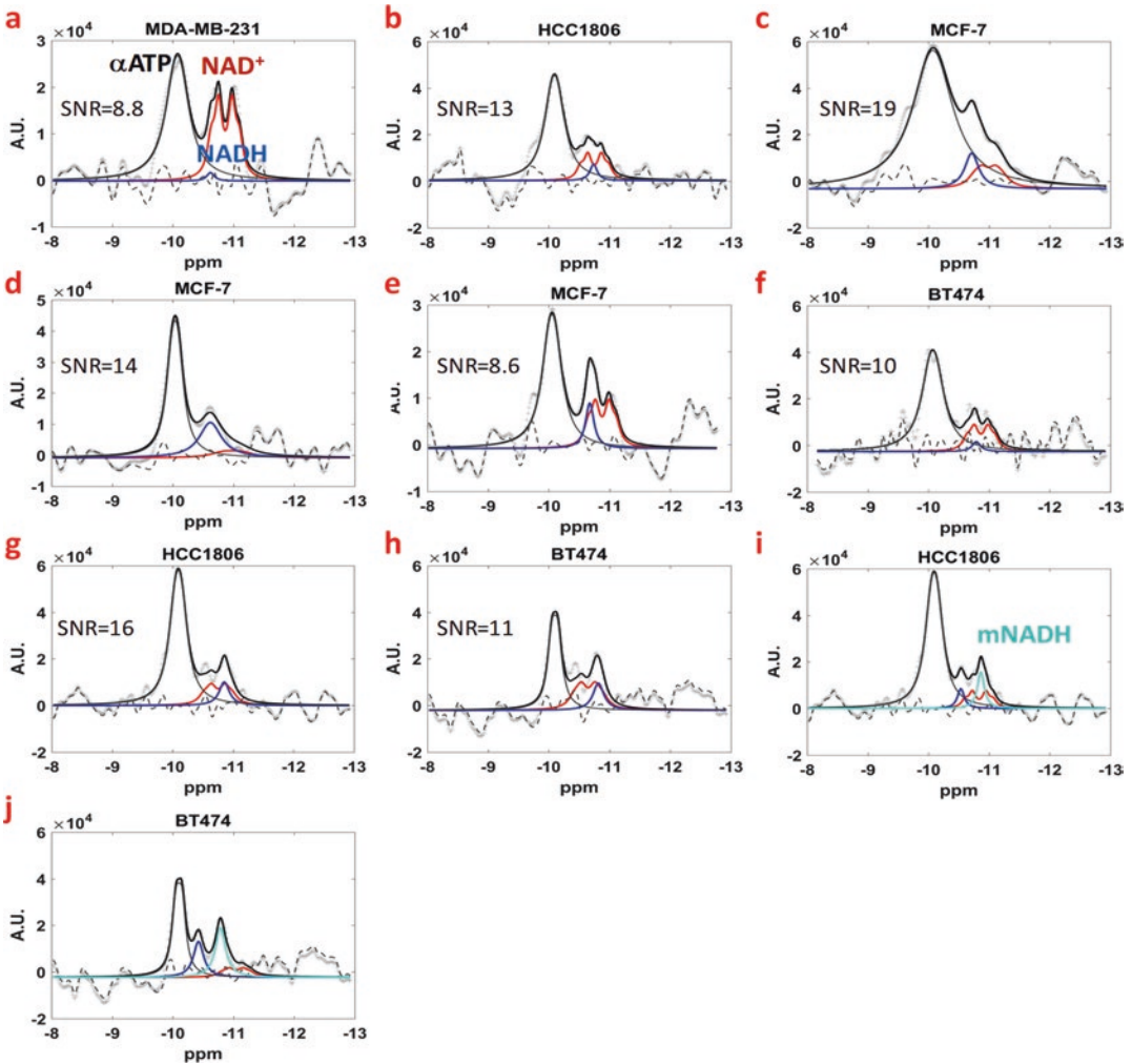
Fig. 1 Spectral fitting of the \alpha ATP region of the ^{31}\text{P} -MRS spectra from breast cancer mouse xenografts. (a–j) Spectral fitting of eight tumors with the names of cancer cell lines and the SNRs displayed on individual spectra. Each spectrum shows the raw data in arbitrary units (A.U.) in light grey, global fit in black, \alpha ATP in grey, \text{NAD}^+ in
