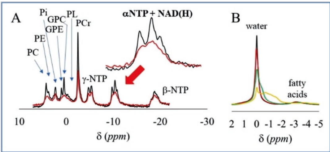
Fig. 1 Non-localised ^{31}\text{P} -MRSI of the head of a healthy human subject. Panel A. Effect of ^1\text{H} irradiation on the ^{31}\text{P} signals (black) vs. no irradiation (red). The inset expands the \alpha\text{NTP-NAD(H)} region. Assignments PC phosphocholine, PE phosphoethanolamine, Pi inorganic phosphate, GPE glycerophosphoethanolamine, GPC glycerophosphocholine, PL phospholipids, PCr phosphocreatine;
