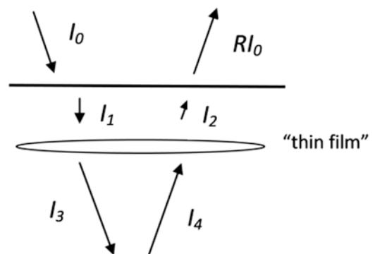
Fig. 1 Four fluxes in a quasi two-layer model
