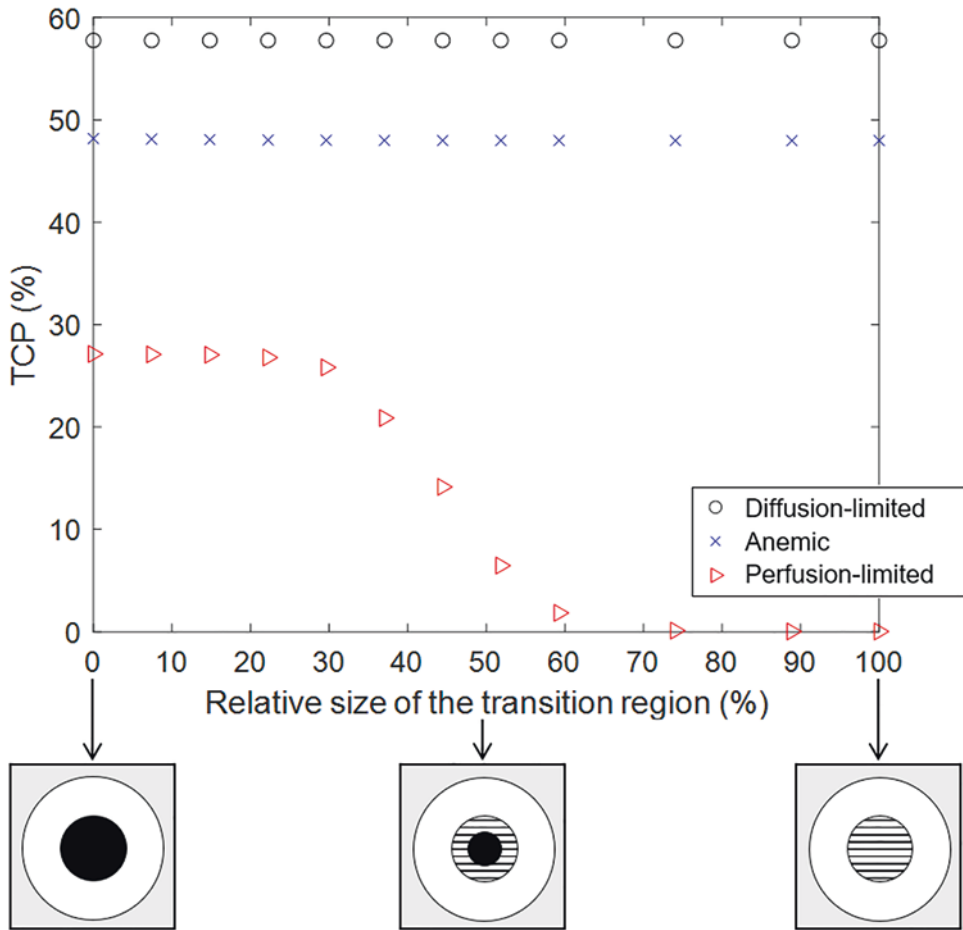
Fig. 2 The TCP for the three modelled tumours after exposure to a dose of 18 Gy, as a function of the radius of the transition region relative to the maximal radius of 1.4 mm
