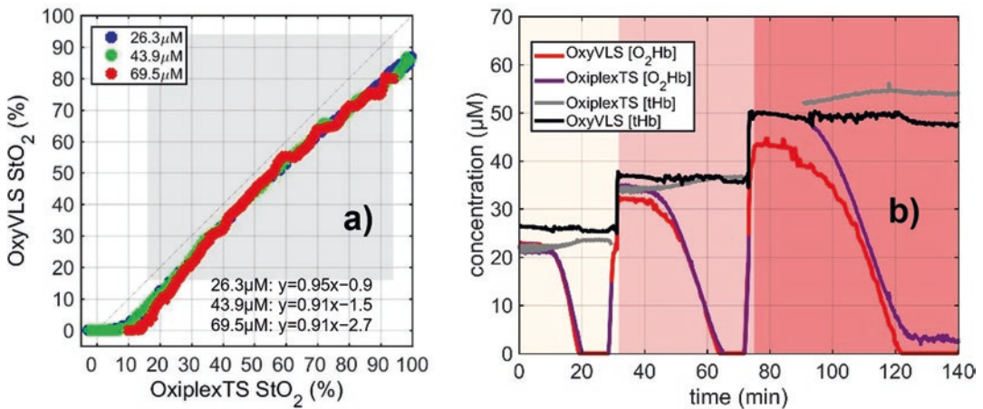
Fig. 2 (a) \text{StO}_2 measured by OxyVLS (y-axis) and OxiplexTS (x-axis) agree well irrespective of the [tHb]. (b) [O 2 Hb], and [tHb] measured by OxyVLS in comparison to OxiplexTS. The shading indicates [tHb] = 26.3 \mu\text{M} , 43.9 \mu\text{M} , 69.5 \mu\text{M} . From 75 to 90 min the OxiplexTS data is missing due to a technical problem
