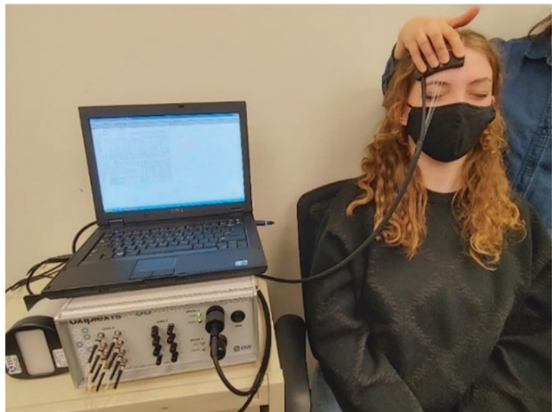
Fig. 1 Frequency-domain near-infrared spectroscopy (ISS OxiplexTS, model 96,208, ISS Inc., Champaign, IL) used in the measurement of frontal cortical microvascular oxygenation ( S_tO_2 )
