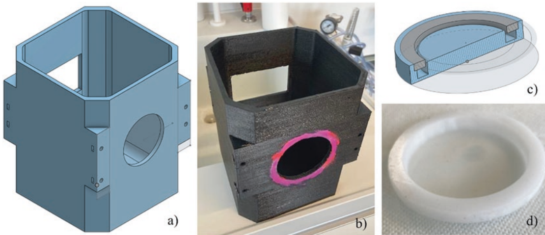
Fig. 1 Liquid phantom container: CAD (a) and photo (b) of phantom. CAD of the mold (c) and a photo of the circular window (d)
