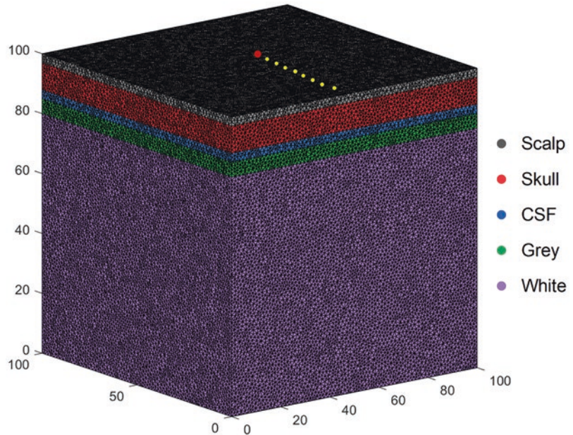
Fig. 1 Mesh slab representing an adult head used for the Monte Carlo simulations
