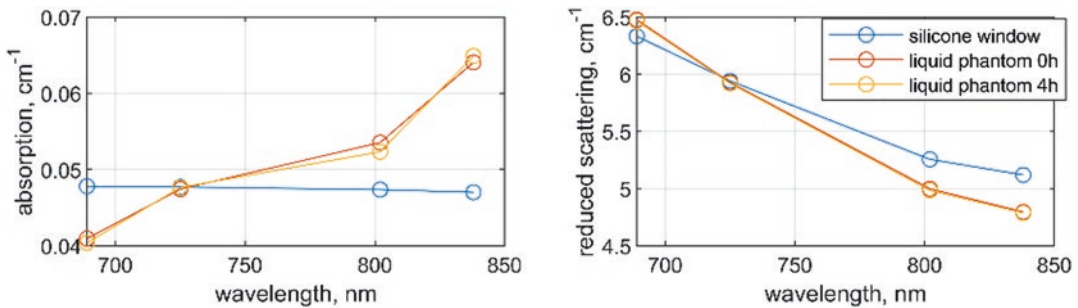
Fig. 2 Optical properties of the silicone window used in this study (blue), and liquid phantom right after preparing the mixture in the phantom container (red) and the same mixture after 4 h at a room temperature (yellow)
