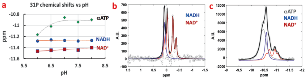
Fig. 2 ^{31}\text{P} -MRS studies of ATP, \text{NAD}^+ and NADH phantoms. (a) pH dependence of chemical shifts in ppm; each point representing a separate phantom using external 85% \text{H}_3\text{PO}_4 as 0 ppm reference; (b) spectral fit for a mixture of \text{NAD}^+ (10 mM) and NADH (10 mM) at pH 6.2, \delta_{\text{NADH-NAD}} = 0.22 ppm; (c) spectral fit for a mixture of ATP
