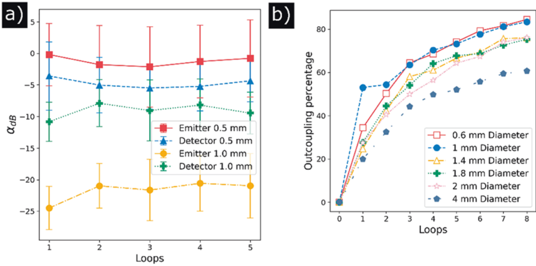
Fig. 1 (a) Different numbers of loops and diameters show different attenuation compared to baseline measurements. (b) Outcoupling percentage as a function of the number of loops and loop diameter
