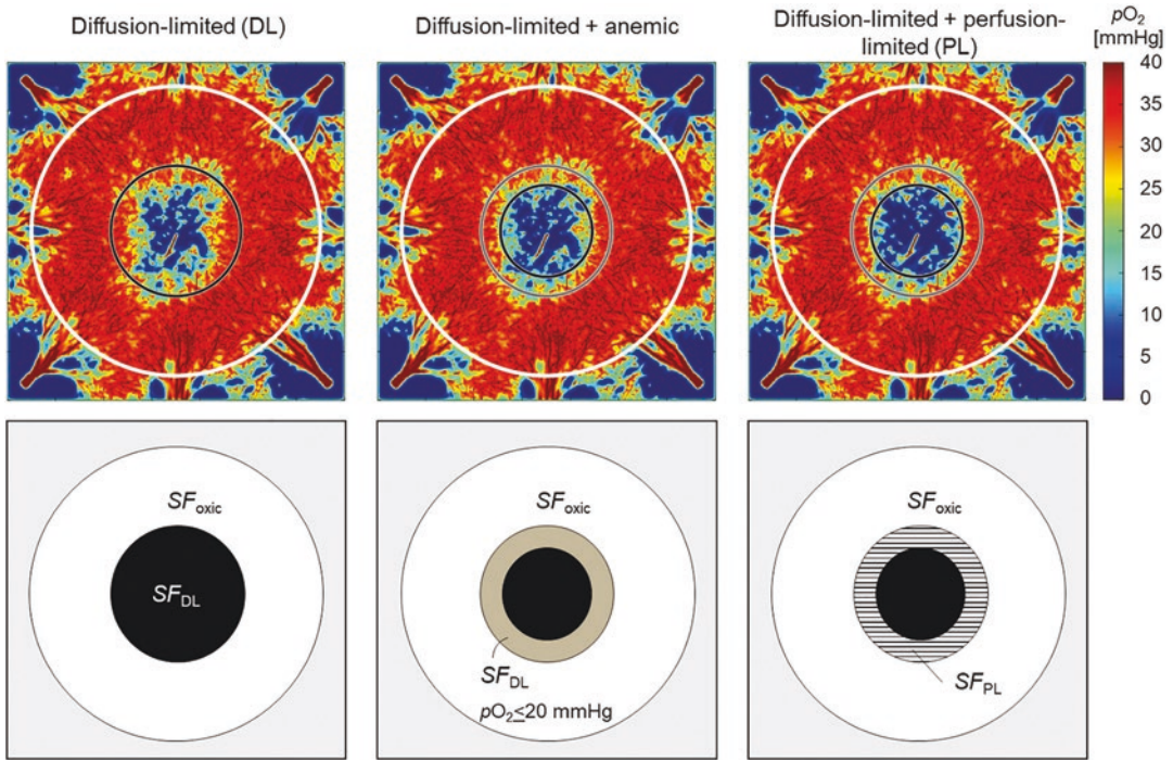
Fig. 1 Cross-sections of the tumour models showing the pO_2 maps (upper panel) and the regions in which the different expressions for calculating the cell survival were used (lower panel)
