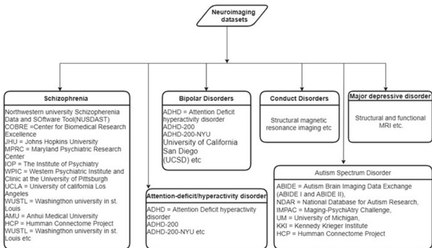
Fig. 2 Neuroimaging datasets
