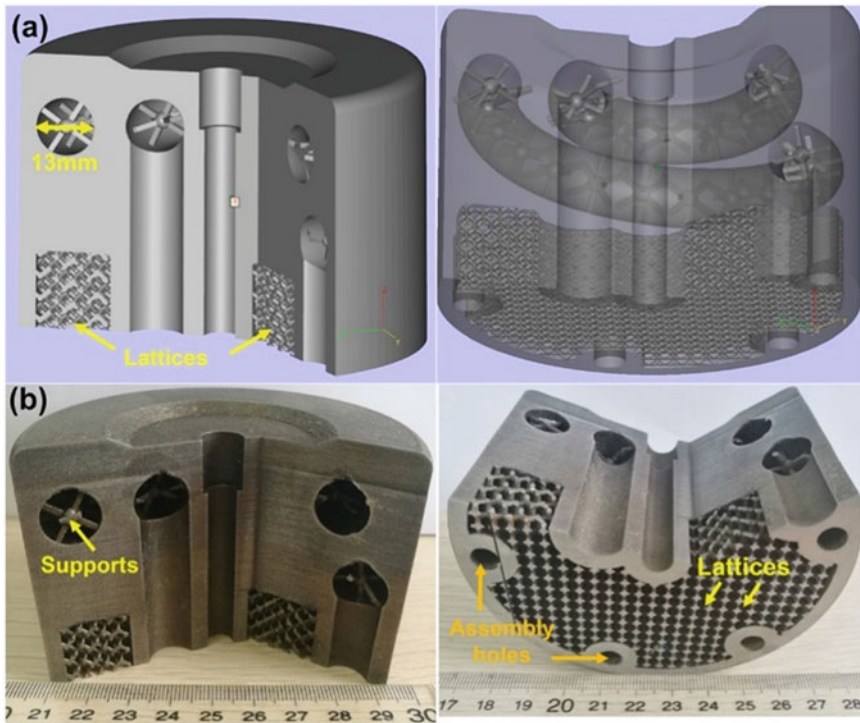
Fig. 6.34 Novel Conformal cooled mould insert: a CAD models of novel conformal cooled mould insert, b the corresponding mould insert processed by PBF-LB/M (Reprinted from Materials and Design , Vol. 196/109147, Chaolin et al. [10], Copyright 2021, with permission from Elsevier)
