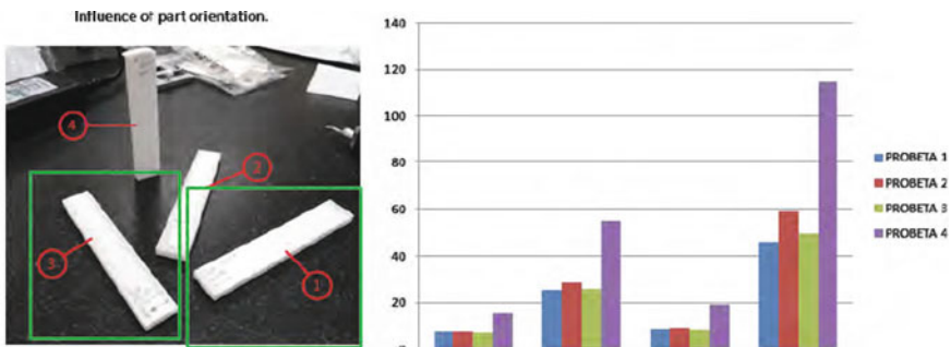
Fig. 7.56 Surface roughness in LS parts positioned in different reference axis (Source Skin project, AIDIMME)
