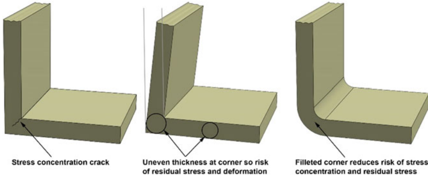
Fig. 4.22 Example of simple filleting to eliminate both stress concentrations and residual stress (Courtesy of Olaf Diegel [1])
