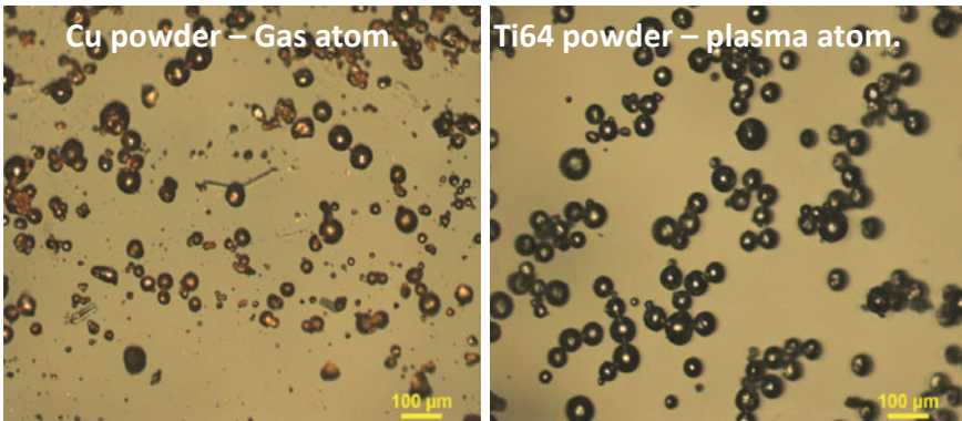
Fig. 7.17 Copper (on the left) and Ti6Al4V (on the right) powder particles produced by gas and plasma atomization, respectively (Source AIDIMME)
