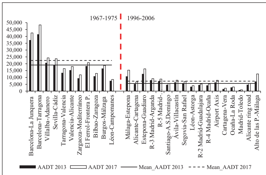
Fig. 2 Traffic demand in 2013 and 2017 comparison between toll motorway awarded in 1967–1975 and toll motorways awarded in 1996–2006
