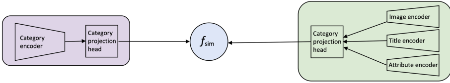
Fig. 1. Overview of CLIP-ITA. The category encoding pipeline is in purple; the category information pipeline in green; f_{sim} is a cosine similarity function. (Color figure online)
