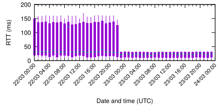
Fig. 8. Anycast B and Comcast: RTT before and after resolving IPv6 misconfiguration.
