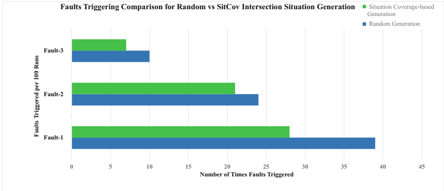
Fig. 11. Faults triggering of SitCov-based vs random intersection situation distribution generation
