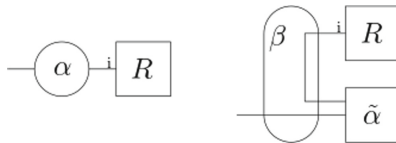
Fig. 1. On the left, the converter \alpha is connected to a resource R . On the right, the interpretation where the converter \alpha is interpreted as a resource \tilde{\alpha} in parallel, with a trivial converter that connects interfaces.
