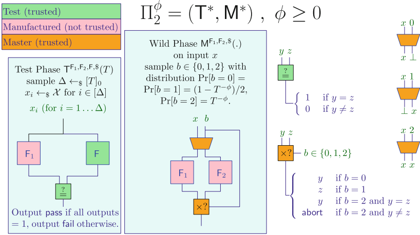
Fig. 4. Construction \Pi_2^\phi from Conjecture 1.
