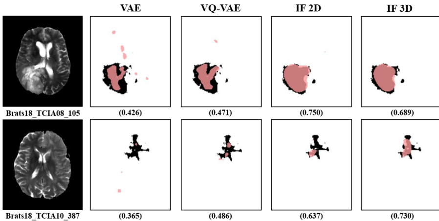
Fig. 3. Visual comparison of anomaly scores (pink) versus ground truth (black) for two different subjects (central axial slice). In brackets, DICE score for the whole subject. (Color figure online)
