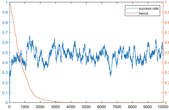
Fig. 2. Development of CRS for the Trid Hessian H_{T10} . In orange the reached function value of the worst point in the population and in blue the success rate.
