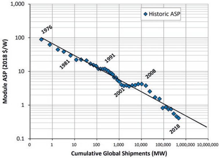
Fig. 16.2 Decreasing investment prices for solar photovoltaics modules. (Source: Paula Mints 2019)
