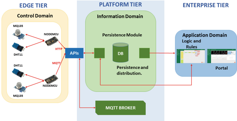
Fig. 2. Proposed IoT indoor application.
