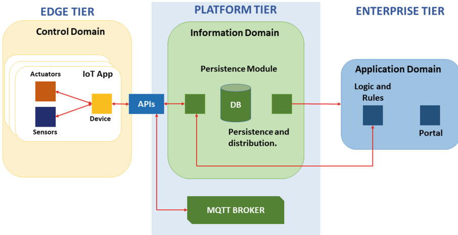
Fig. 1. Designed architecture for the system based on [8]
