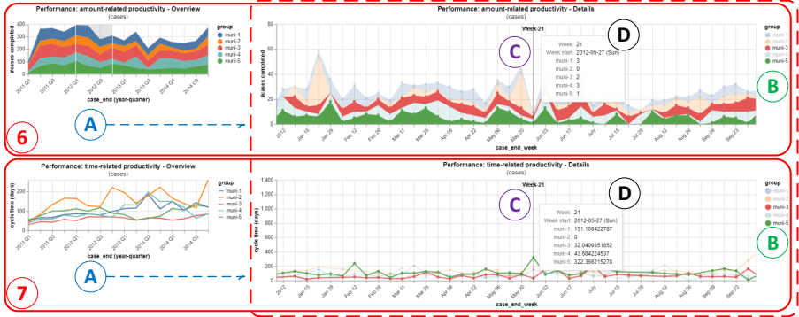
Fig. 3. Annotated screenshots of the prototype’s interface for analyzing work profiles regarding performance. Views of (6) amount-related productivity and (7) time-related productivity respond simultaneously to user interactions (A–D)
