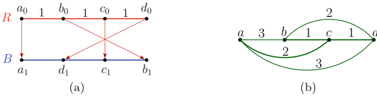
Fig. 1. Four points that move from time 0 to time 1. (a) R is the MBST at time 0, and B is the MBST at time 1. (b) The graph G ; green edges form an MBMST of this graph. (Color figure online)
