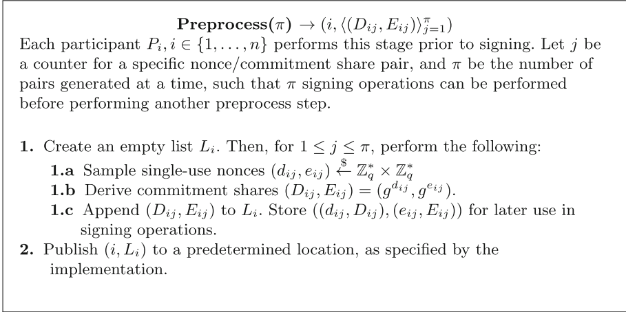
Fig. 2. FROST preprocessing protocol
