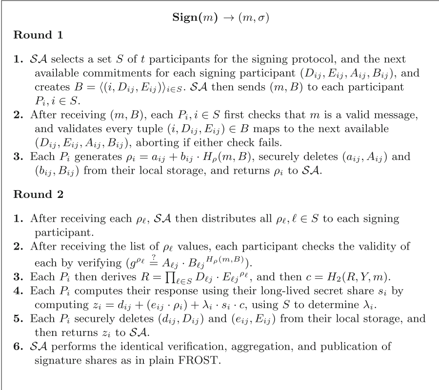
Fig. 5. FROST-interactive two-round signing protocol
