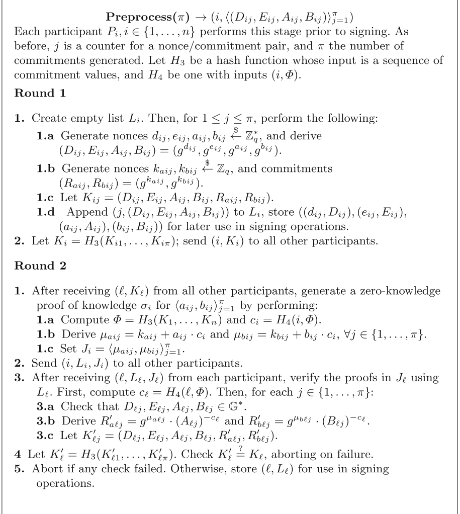
Fig. 4. FROST-interactive two-round preprocessing protocol
