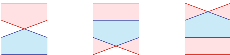
Fig. 16 Normal rulings near a switch
