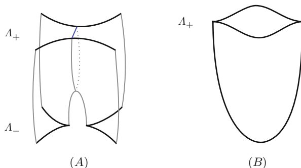
Fig. 1 (a) The pinch move on \Lambda_+ produces a Lagrangian saddle; (b) \Lambda_+ obtained by introducing an unknotted component to \Lambda_- corresponds to the Lagrangian cobordism having a local min
