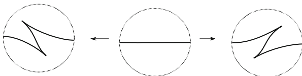
Fig. 4 Two ways to stabilize a Legendrian knot in the front projection
