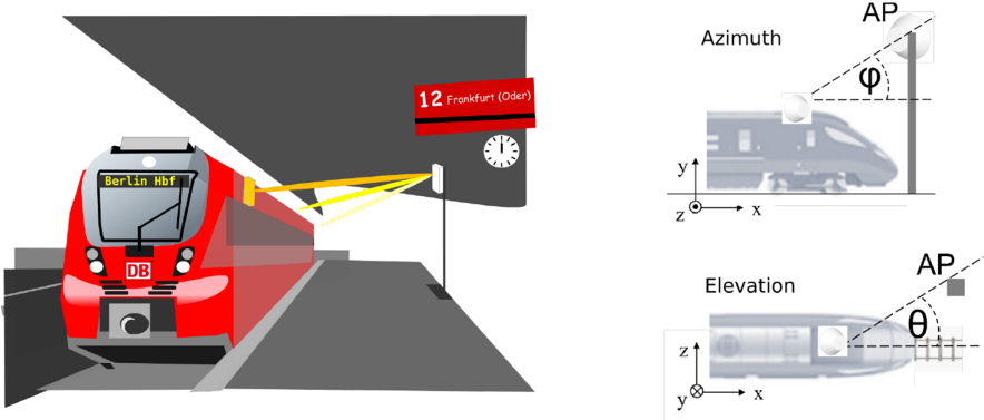
Fig. 4. a) Sketch of the track-to-train communication using mmWave pencil beams b) Azimuth and elevation requirements depending on the angles, COTS hardware used for the trial.
