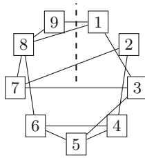
Fig. 1. Illustration of Definition 6 on a graph G with n = 9 with a cb-labeling \varphi such that B_c(G, \varphi) = 4 . Each edge uv crossing the dashed vertical line has a non-zero \alpha_\varphi(u, v) .
