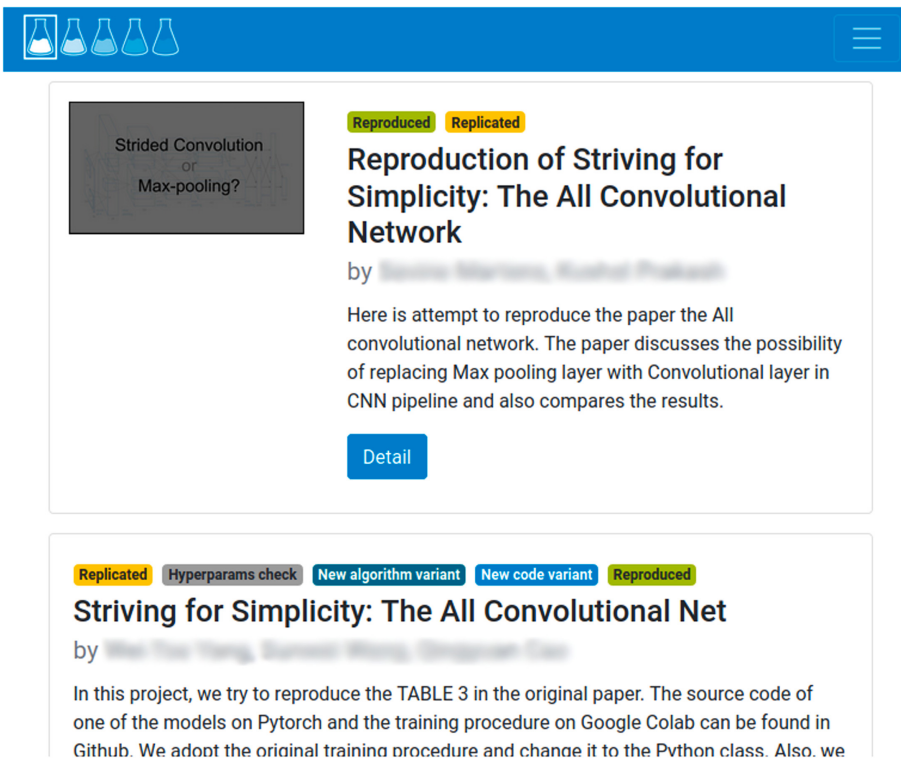
Fig. 1. A screenshot of ReproducedPapers.org . We allow multiple reproductions of the same original paper and investigations of several aspects, such as Reproduced , Replicated , Hyperparameter check , etc. Our online repository is user-centered: its sufficient if a user sees value in uploading some form of reproduction. Having such a repository is well-suited for students and adds structure to reproducibility in machine learning.
