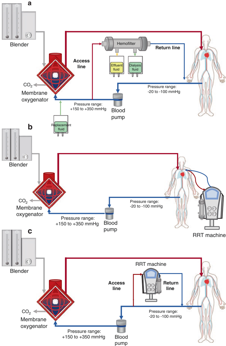
Fig. 18.1 Options for combining extracorporeal membrane oxygenation (ECMO) and continuous renal replacement therapy (CRRT) circuits. (a) An in-line hemofilter is integrated into the ECMO circuit. Replacement fluid is directly administered into the ECMO circuit. Alternatively, dialysis fluid can be supplied in a counter-current position. Replacement/dialysis fluid rates and ultrafiltration rates can be controlled via infusion pumps. (b) The CRRT device is connected to the patient through a separate catheter independent of the ECMO circuit. (c) The access (inlet) and the return (outlet) lines of the CRRT device are connected before the centrifugal blood pump (low-pressure part) of the ECMO circuit. (d) Both the access and the return lines of the CRRT device are connected after the blood pump. (e) The access line of the CRRT device is connected directly after the membrane oxygenator, while the return line is connected directly before the oxygenator
