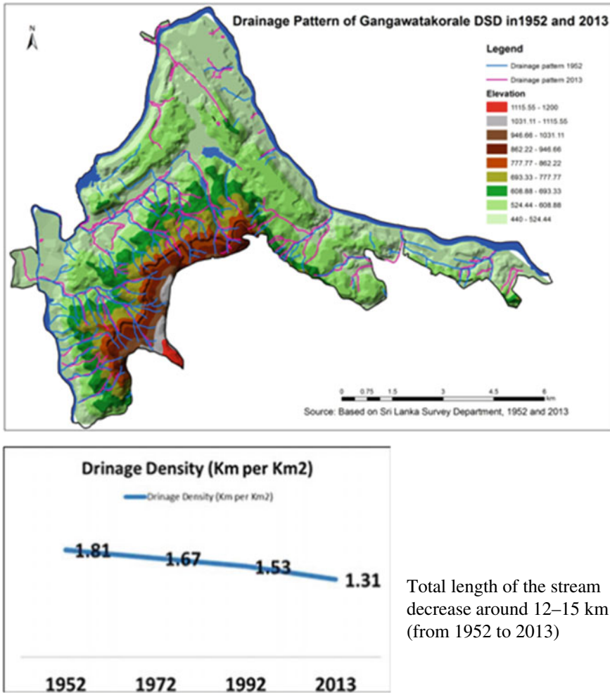
Fig. 2 a Map showing the drainage pattern of Gangawatakorale DSD in 1952 and 2013. Design by Lalitha Dissanayake and Nilukshi Perera, b Graph showing the decreasing pattern of drainage density in Kandy Meda Ela from 1952 to 2013 (Dissanayake 2016)
