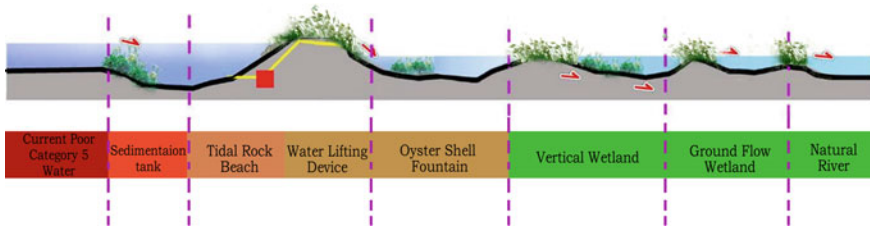
Fig. 6 Process of water purification in the Haizhu Wetland. (Source sorted out from Guangzhou Municipal Government (2012) by the authors) (The image demonstrates the process of water purification in Haizhu wetland. There are 7 steps to achieve water purification. The first step is to divert the poor category five water from sewage near the Haizhu wetland to the sedimentation tank. The second step is to filter the coarse particles in the poor category five water through the natural sedimentation and physical adsorption. The third step is to pass the water in the sedimentation tank through the tidal rock beach, filter the small particles of impurities, and to introduce it into the wetland through the pumping equipment. The fourth step is to increase the oxygen content of the water by stonewall waterfall purification to remove the eutrophic substances in the water. The fifth step enters the vertical flow wetland, reduces the nitrogen and phosphorus content in the water through the absorption of the wetland vegetation with the drop. The sixth step is ground flow wetland, through the biological comprehensive purification to improve water quality. The seventh step is to enter the natural rivers of the large water surface, where the water quality is basically restored to the second water, which is available for landscape water)
