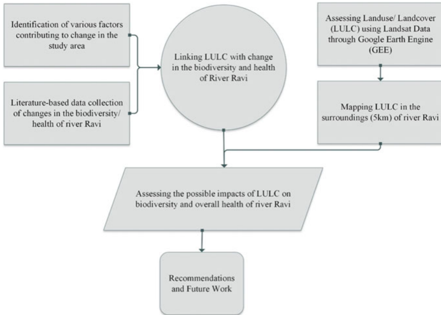
Fig. 2 Proposed methodology for the assessment of LULC on river overall health and biodiversity
