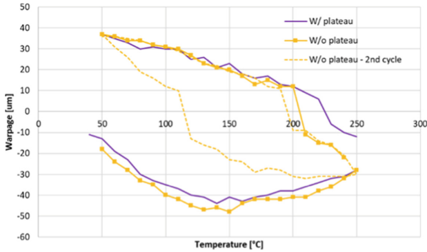
Fig. 2. Measured warpage during temperature profiles. Negative values are reached during the heating, while positive ones during the cooling phase. Dotted line represents the warpage vs temperature profile occurred during a second temperature cycle.
