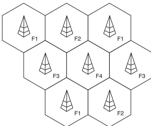
Fig 17.2 Frequency reuse in cellular networks
