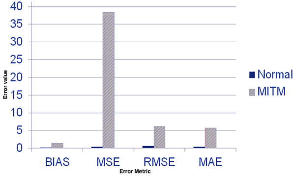
Fig. 7. Reconstruction error between normal and attack patterns using LSTM.
