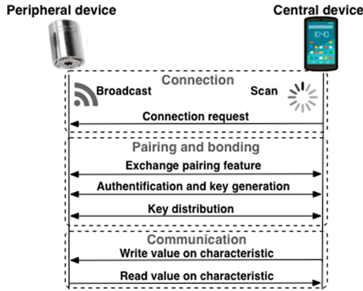
Fig. 1. BLE workflow between peripheral and central devices.
