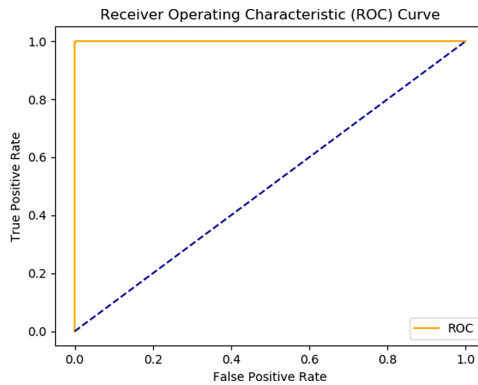
Fig. 10. ROC curve of the BLE packets classifier.
