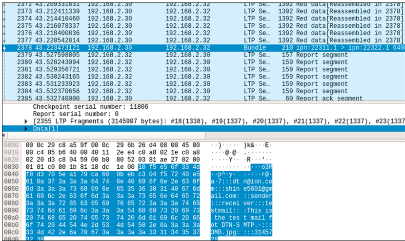
Fig. 6. LTP communication between DTN nodes
